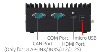
DLAP-211-JNX/Nano (backside)
